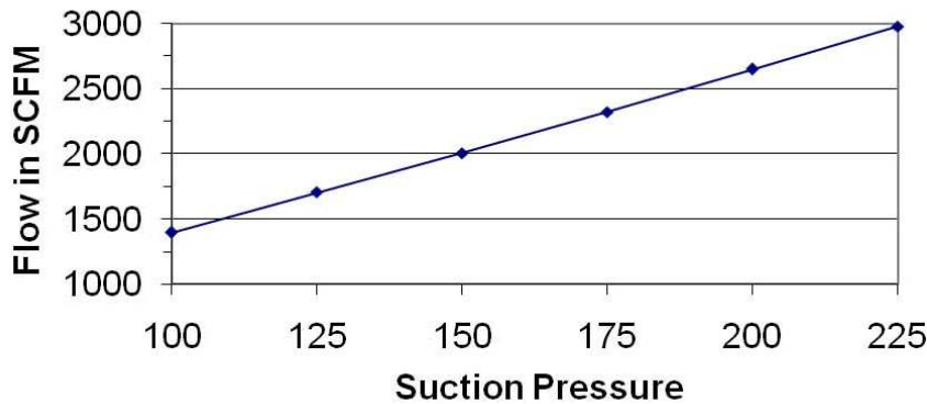
Flow in SCFM vs Suction Pressure With Maximum Discharge Pressure 2-Stage
